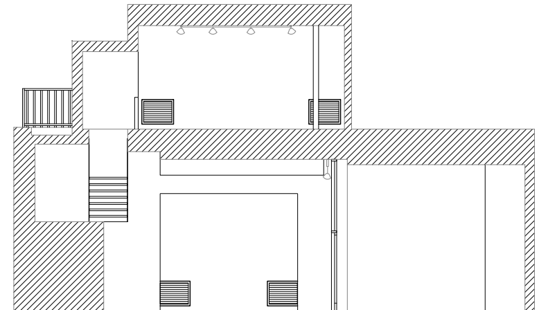
Section CC'
